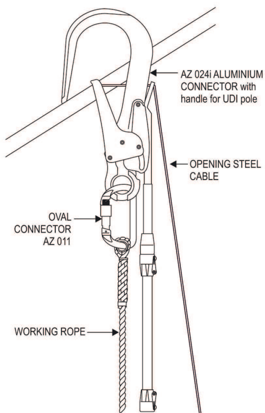
Assembling AZ024 installer on pole
